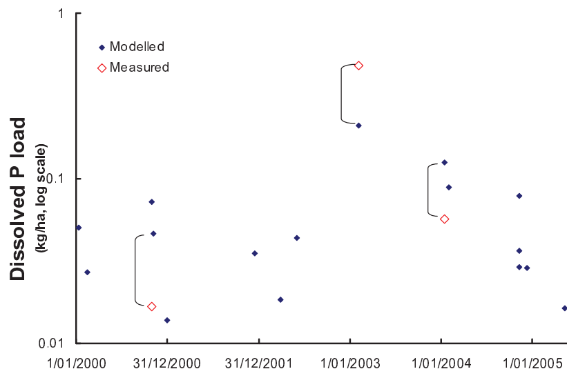
Figure 4. Modelled and measured loads of dissolved P at the Brigalow Catchment Study. For the three measurements, the modelled data are linked by a “[“.
