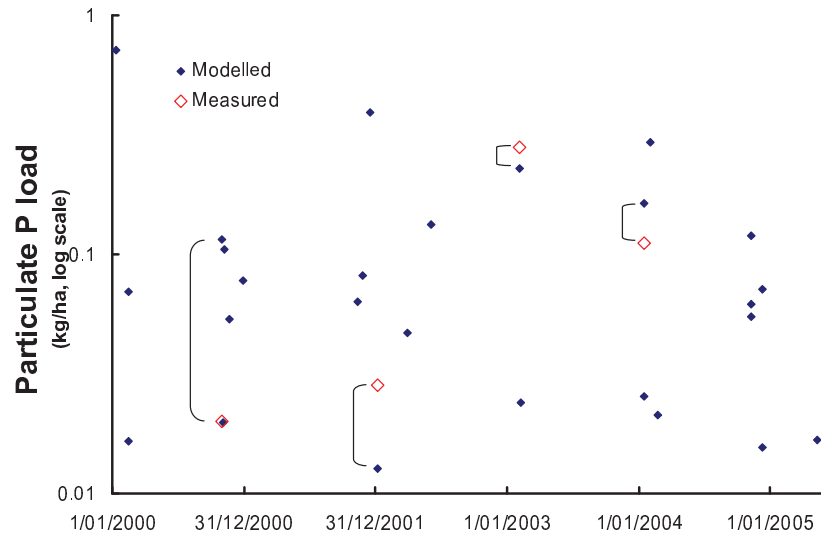
Figure 5. Modelled and measured loads of particulate P at the Brigalow Catchment Study. For the 4 measurements, the modelled data are linked by a “{”.
